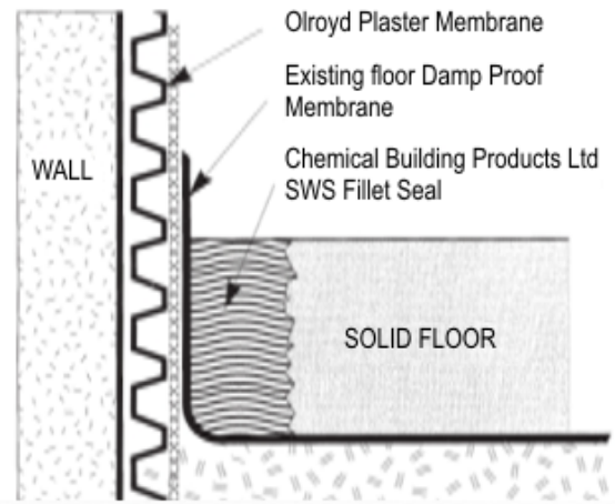
DIAGRAM 2 Oldroyd Plaster Membrane Plug and Compression Seal
