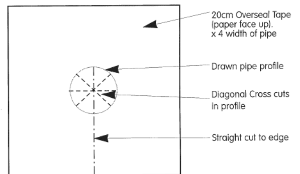
DIAGRAM 6 Incoming Service Collar
